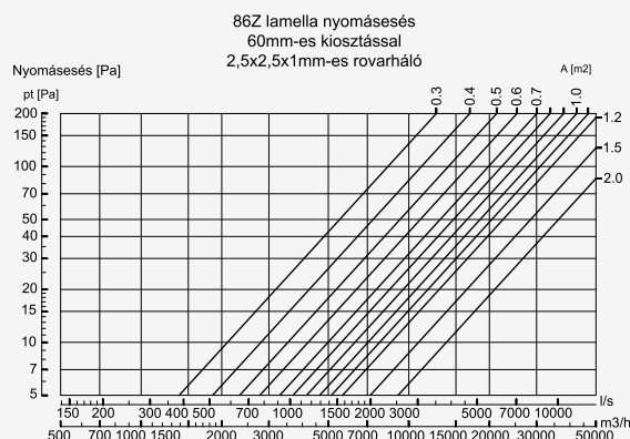
Lamella
