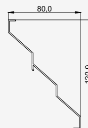
Lamella
